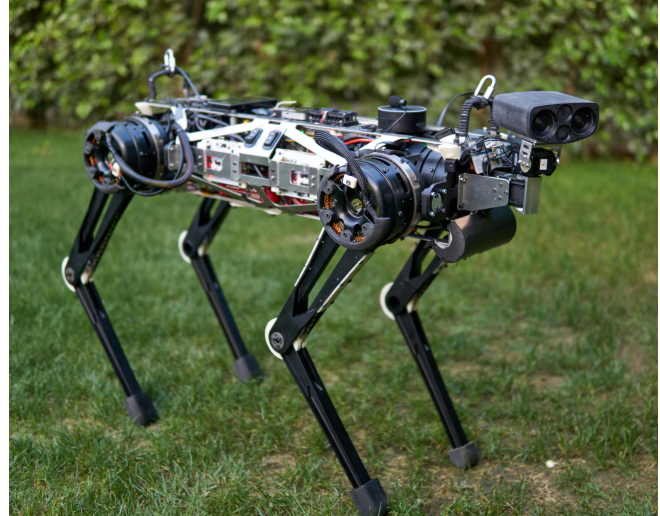
Fig. 1: MIT Cheetah 3. The MIT Cheetah 3 quadruped robot platform is an electrically powered robust robot capable of untethered 3D locomotion in uncertain terrains.
